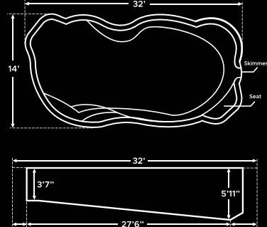
The Santa Fe
