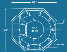
The Flagstaff 36" Deep Octagon
