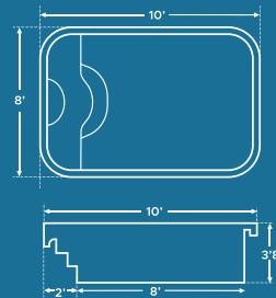
The Dallas 44" Deep Rectangular Spa
