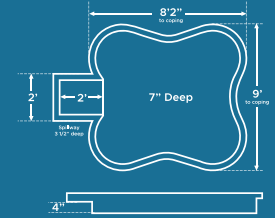
The Arlington Tanning Ledge
